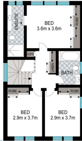
UPPER LEVEL
