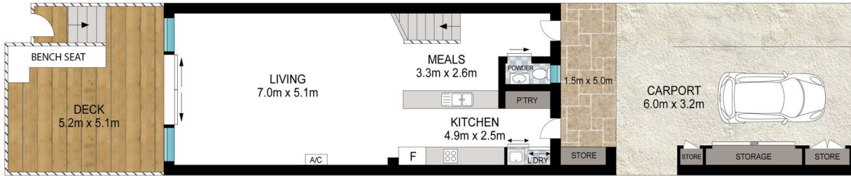
GROUND FLOOR
