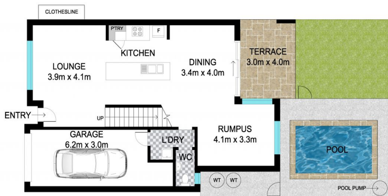
LOWER LEVEL
